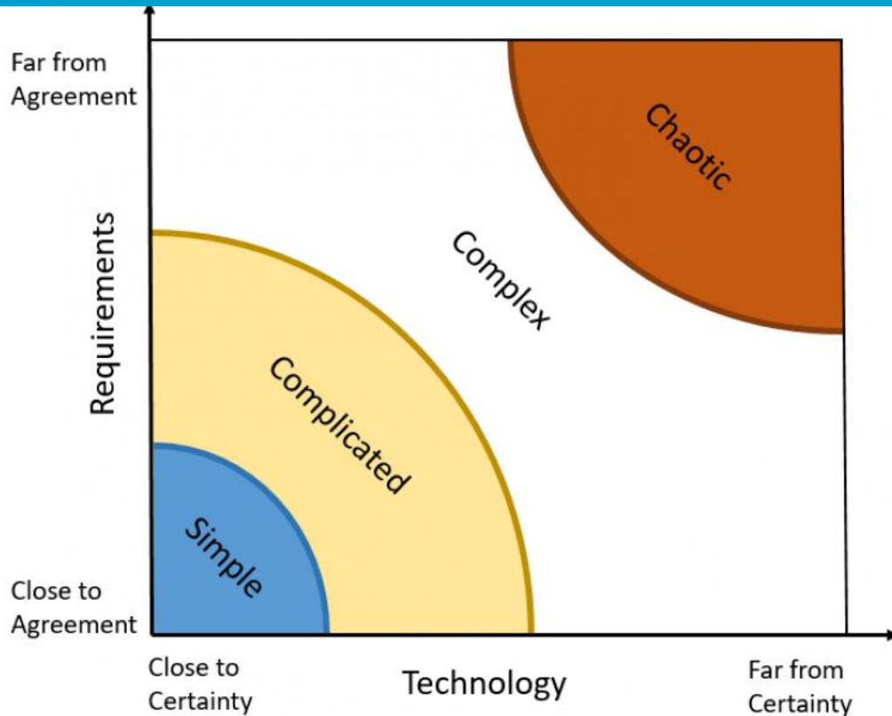
Stacey matrix
